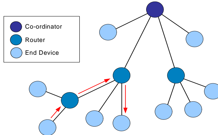
Figure 7: Tree Network
