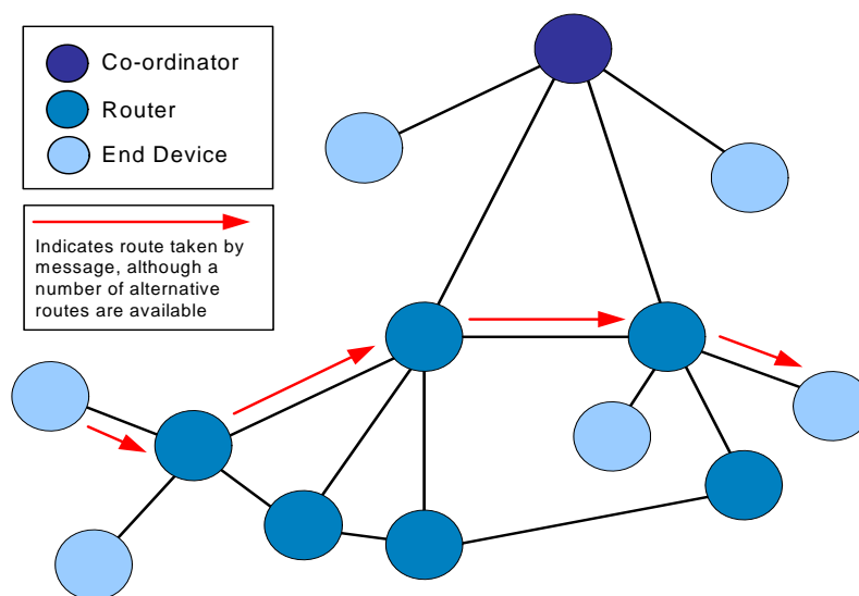
Figure 8: Mesh Topology
